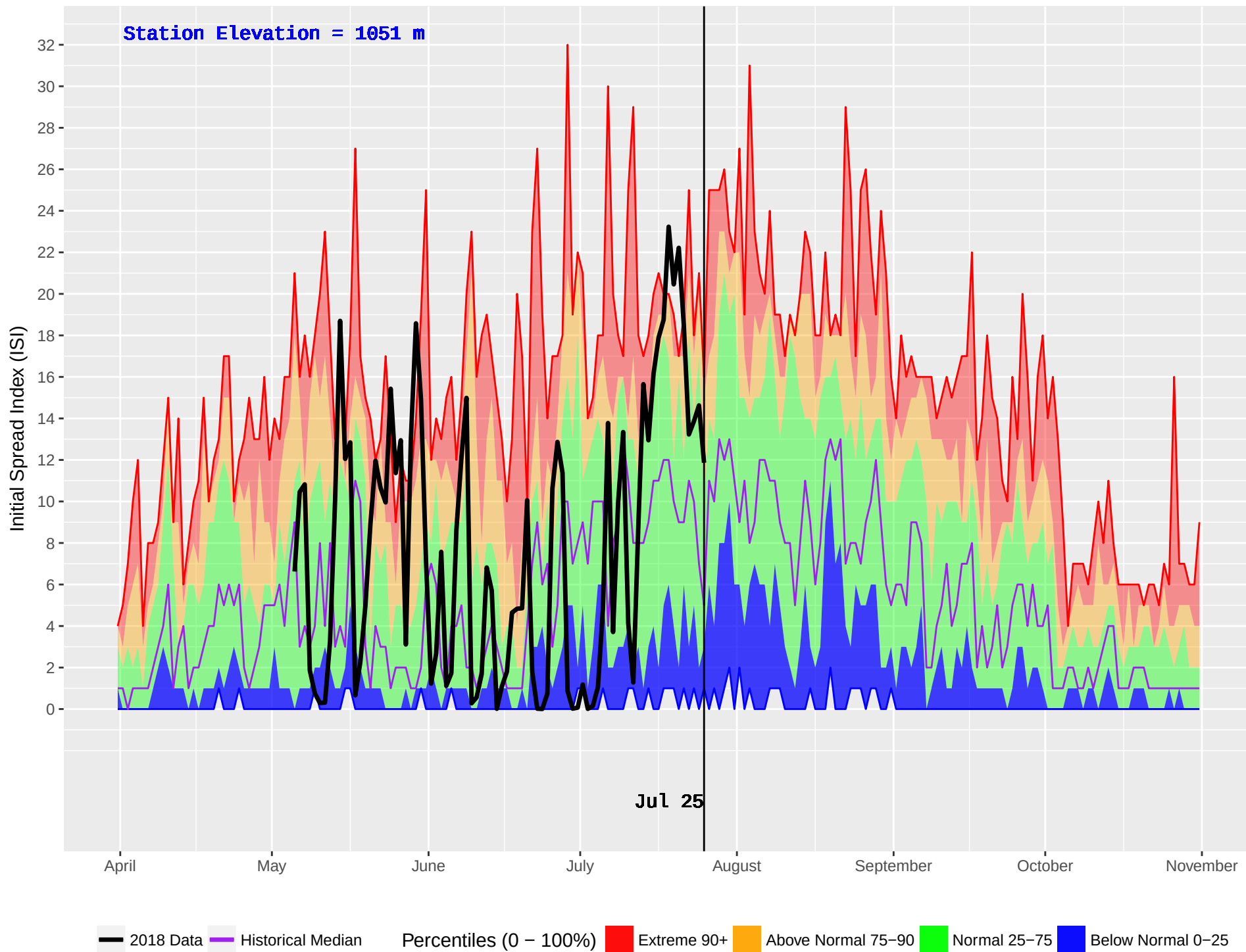
GOATHAVEN (886) : Historical (2005–2016) and Current (2018) Noon Initial Spread Index (ISI)
