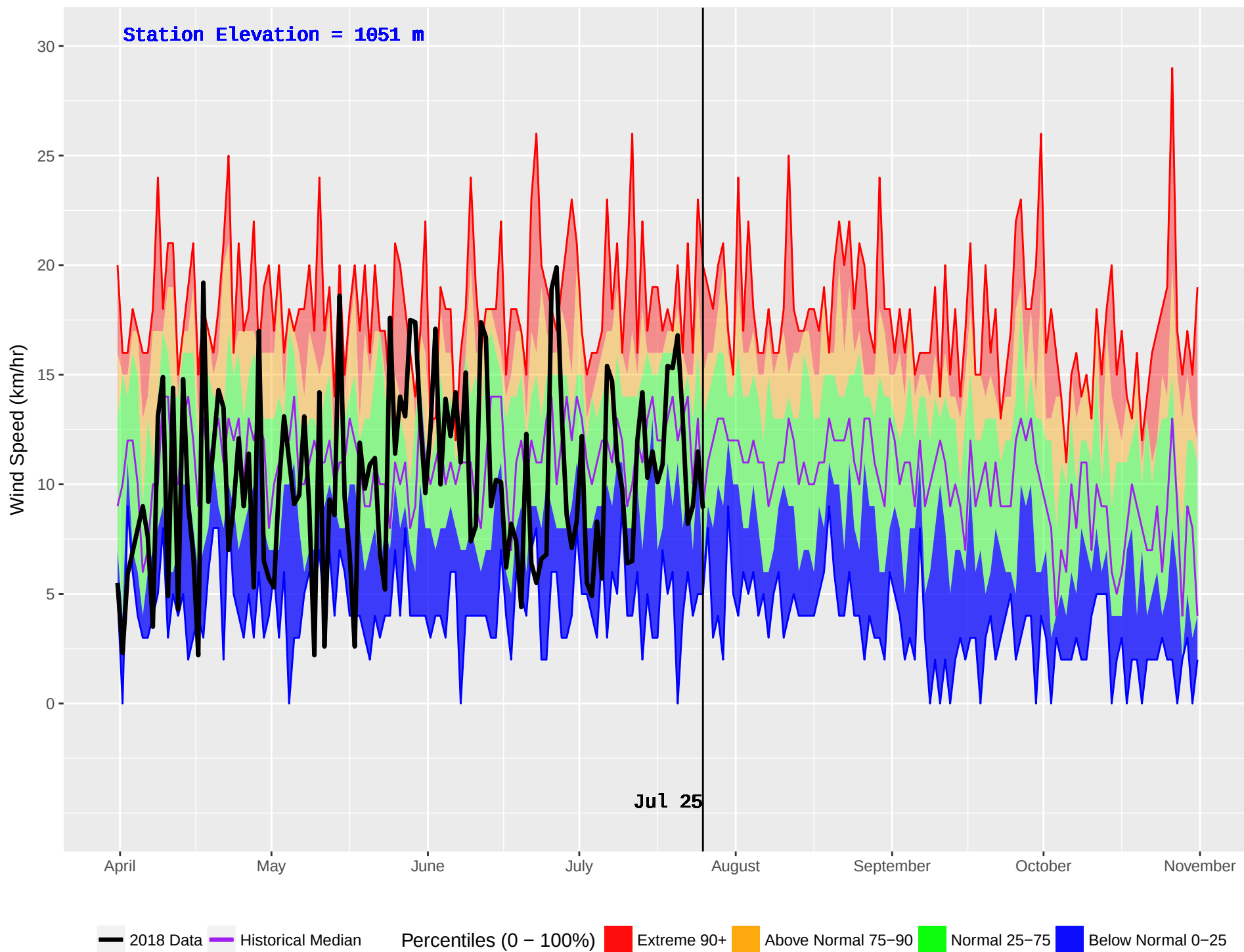
GOATHAVEN (886) : Historical (2005–2016) and Current (2018) Noon Wind Speed
